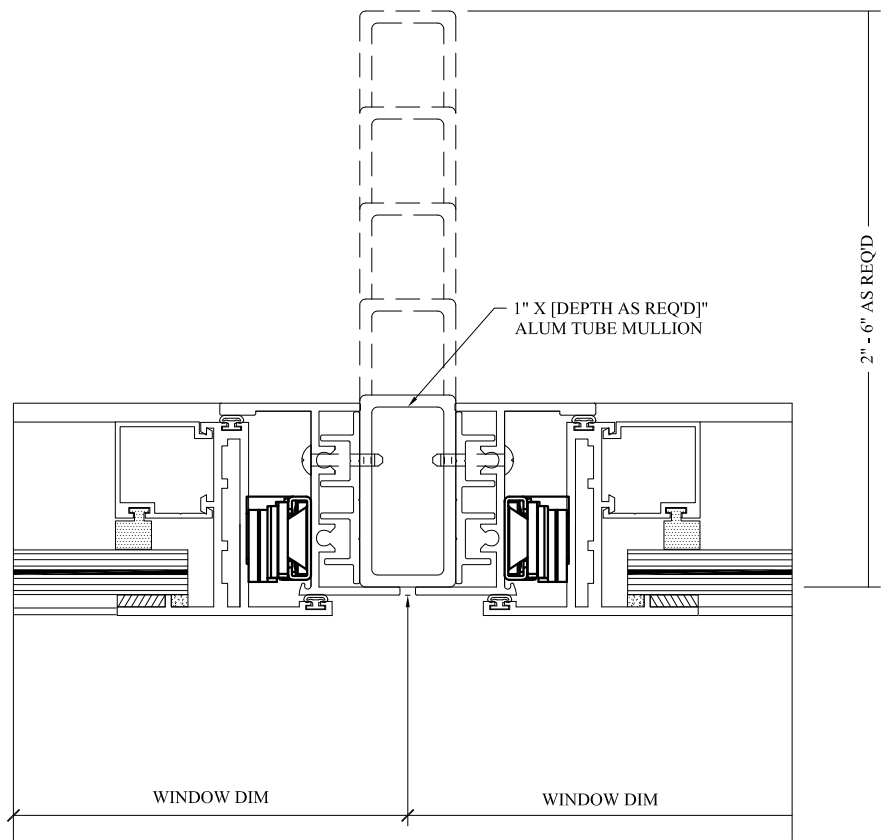
4 TUBE MULLION OPTION SUPERIOR SERIES 300 PROJECT OUT-IMPACT EQUAL LEG - 9/16" GLASS
