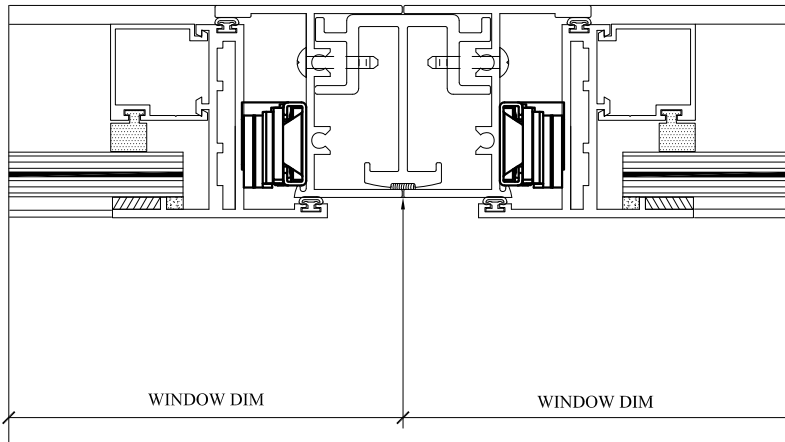
5 ZERO MULLION SUPERIOR SERIES 300 PROJECT OUT-IMPACT EQUAL LEG - 9/16" GLASS
