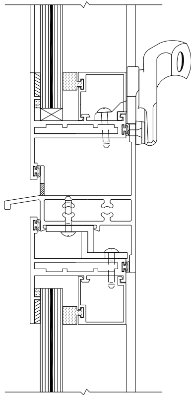
3 MEETING RAIL SUPERIOR SERIES 300 PROJECT OUT-IMPACT EQUAL LEG - 9/16" GLASS
