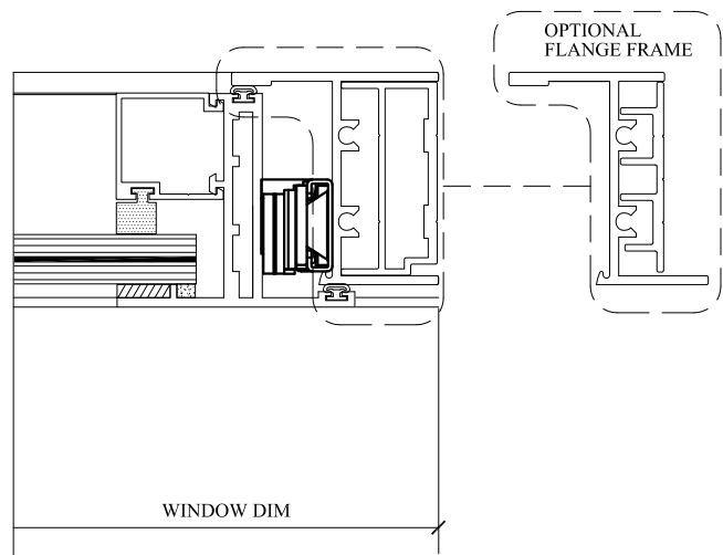
6 JAMB DETAIL SUPERIOR SERIES 300 PROJECT OUT-IMPACT EQUAL LEG - 9/16" GLASS
